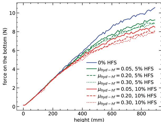
Fig. 16 Force acting on the bottom plate as a function of the bed height (numerical data, orifice size D = 12 mm; cf. experimental data in Fig. 3).
