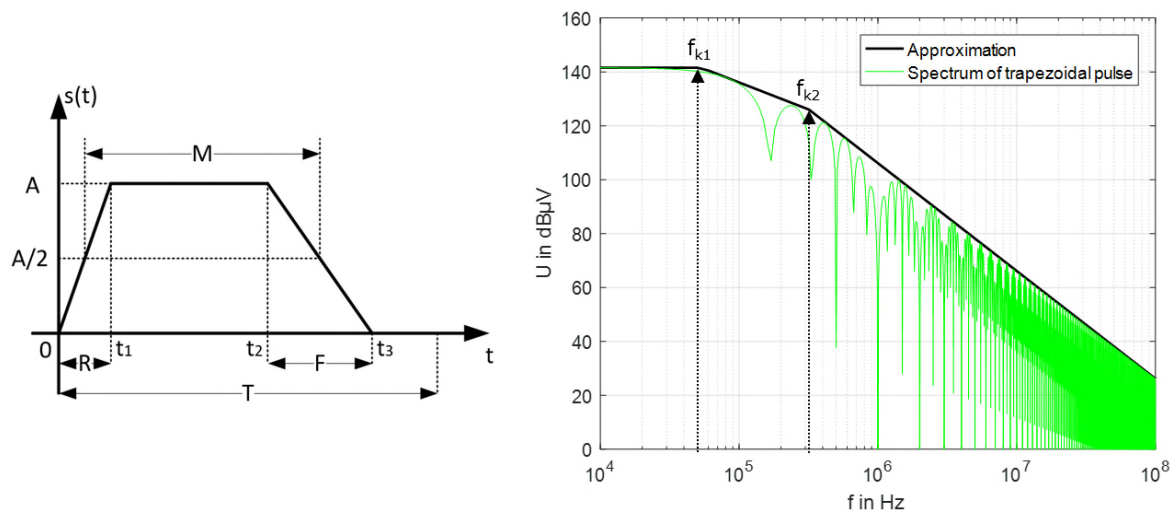
Fig. 2-4: Definition of the trapezoidal pulse in time-domain (left) and its spectrum in frequency-domain in two representations (right)
