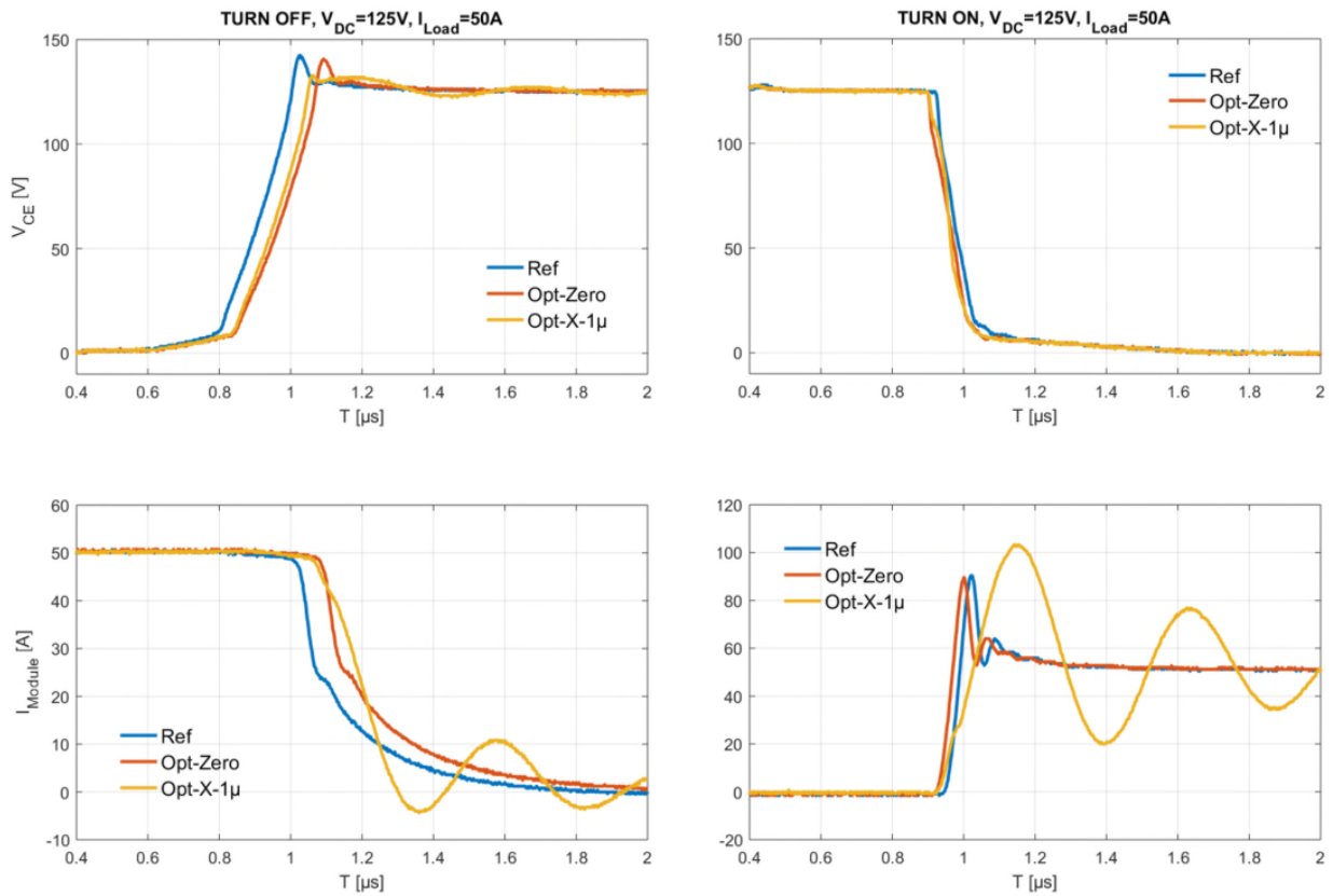
Fig. 6-14: Comparing the switching behavior of the variants group 1: “Opt_Zero” (red) and “Opt_X_1μ” (orange) to the standard HP2 as reference (blue)
