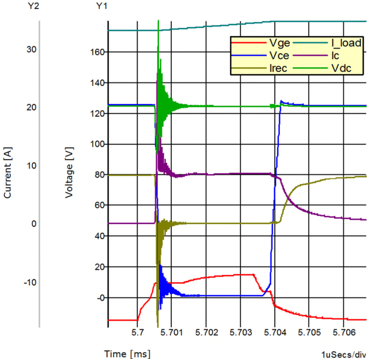
Fig. 4-10: Simulated, more realistic switching curves from the refined simulation model (Tj = 25°C)
