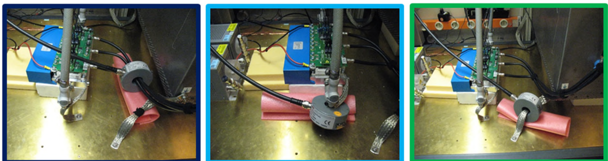
Fig. 4-3: Measurement of the common-mode interference currents: HF current clamp on the AC cables (left); on the ground straps of the power electronics (medium) and the load box (right)
