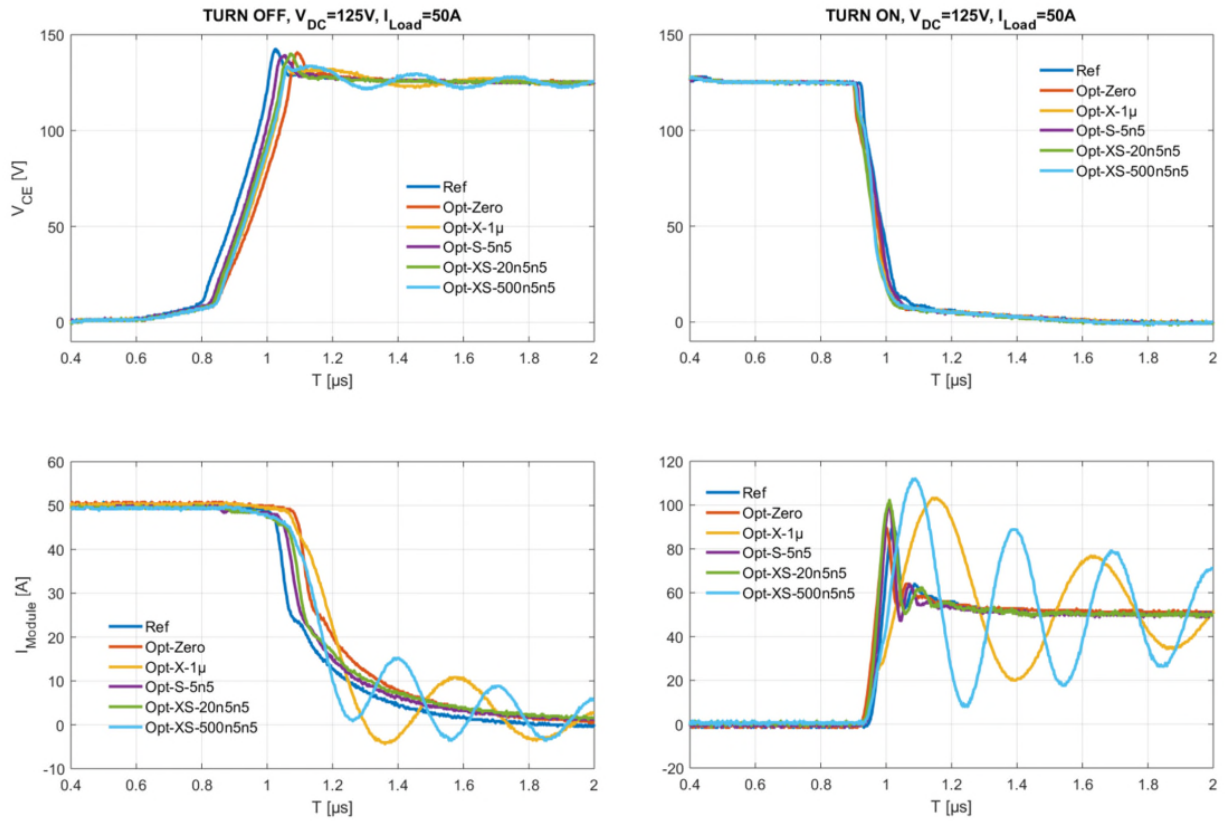
Fig. 6-18: Comparing the switching behavior of the variants group 1 (“Opt_Zero”, “Opt_X_1μ”) and group 2 (“Opt_S_5n5”, “Opt_XS_20n5n5”, “Opt_XS_500n5n5”)
