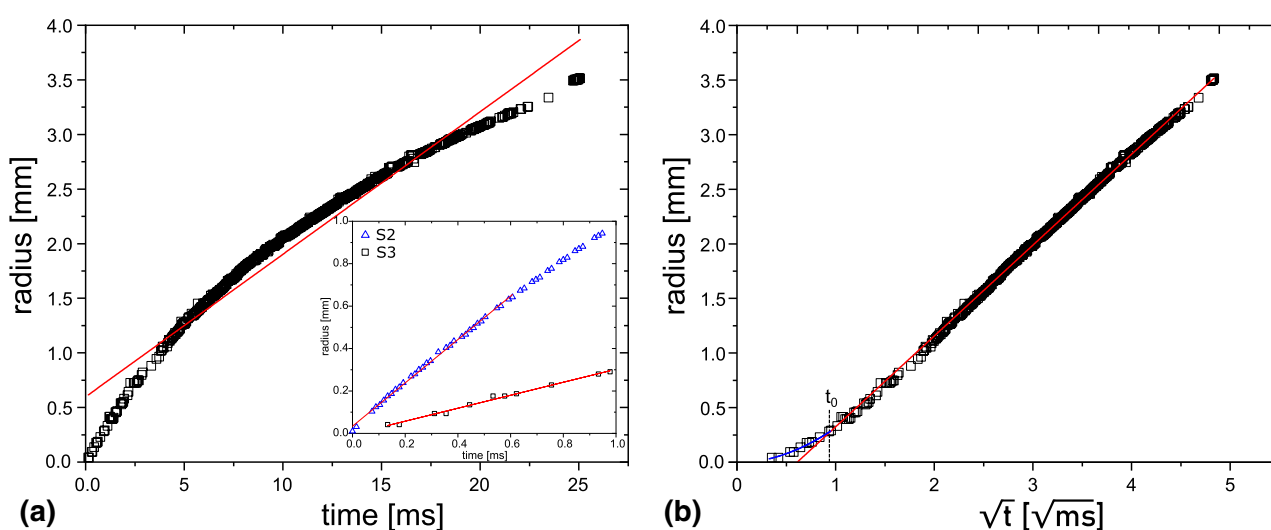
Figure 4. Evaluation of the spreading law exemplary shown for a bubble of solution S3 with R_0 = 6.4 mm on ITO glass: (a) r over t and (b) r over \sqrt{t} . The inset in (a) shows the early time behavior of the spreading for solutions S2 (blue triangles) and S3 (black squares). The cross-over time t_0 is the intersection between the fits of both parts of the curve. The fit of the blue curve is r = at and the red curve follows r = b + c\sqrt{t} .
