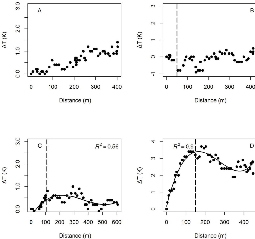
Figure 9. The temperature difference ( \Delta T ) for four green spaces, distinctively showing the high heterogeneity of the temperature gradients found for green spaces in Leipzig (the curve is a polynomial fit and its R^2 value; the dashed line is the park-width distance [PWD]). For (A) (linear) and (B) (flat), no polynomial was fitted. For (A), the transect did not reach up to the PWD.
