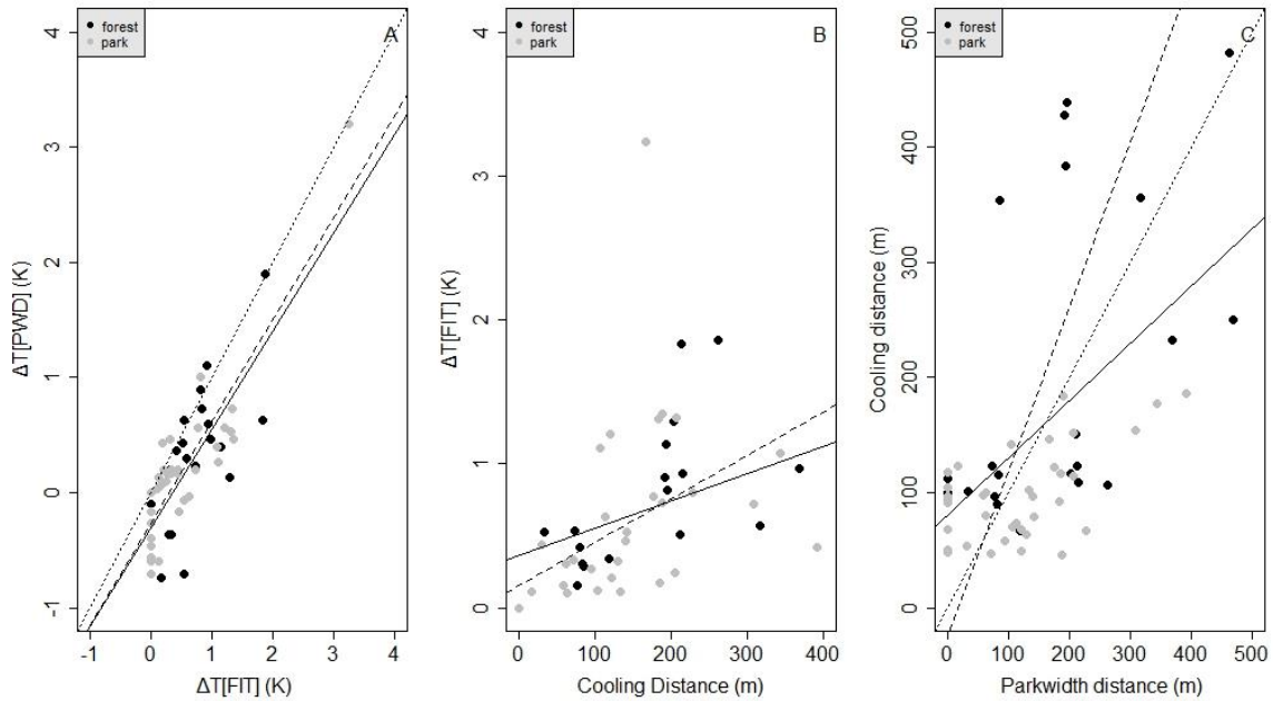
Figure 11. The relationships between the various indicators for quantifying the cooling effect. In A and C, the bisecting line (dotted line) demonstrates perfect agreement of the two different measures of the temperature difference and distances. The lines represent the slopes for the forests (bold line) and the parks (dashed line). B is the calculated cooling effects from cubic polynomial fit. \Delta T[\text{FIT}] is the maximum temperature difference between the green space boundary and the surrounding area measured within the transect route. \Delta T[\text{PWD}] is calculated by subtracting the mean temperature measurement taken at the boundary of the green space from the temperature measured at PWD along the transect, with PWD being the square root of the area of the green space.
