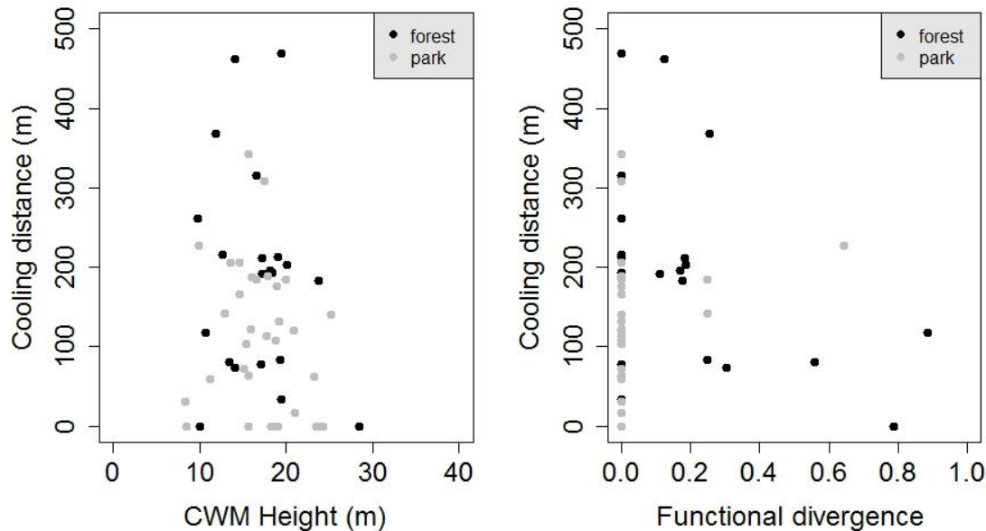
Figure 18. Scatter plots showing the relationship of cooling distance with the CWM height and functional divergence of trees in different types (forests, parks) of UGS.
