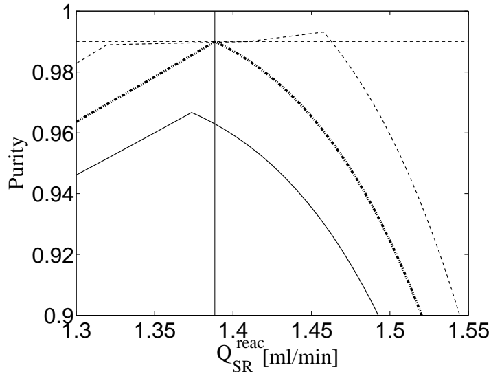
Figure 4.8: Comparison of steady state parameter continuation profiles for nominal, 5%, -5% disturbance of the external feed concentration. The solid lines are for 5%, the dotted lines for nominal and the dashed lines are for -5%. Design without safety margin. Nomenclature same as in Figure 4.2
